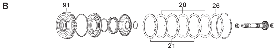
FORWARD CLUTCH & INPUT SHAFT
